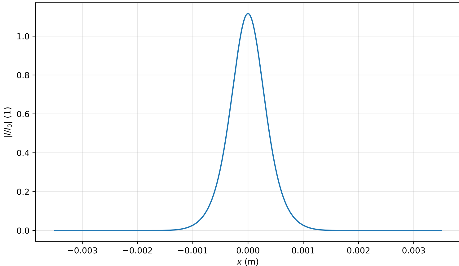
Intensity profile I(x, y = 0, z = 1.115m)/I_0 , P_{in}=0.6P_{cr} , artificial time
